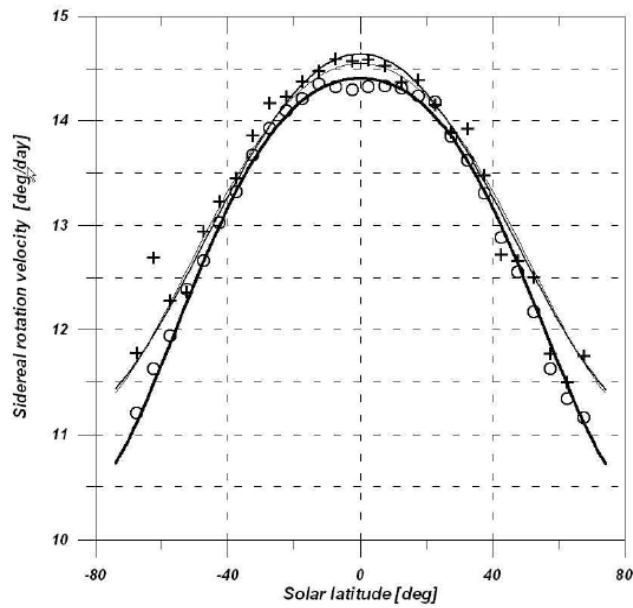
Figure 2.9. Profile of sidereal rotation velocity showing BCG data (circles) and CBP data (crosses). Solid lines show approximations, for o: \omega = 12.183 - \sin^2 b - 1.955 \sin^4 b and for +: \omega = 14.642 - 3.185 \sin^2 b - 0.304 \sin^4 b .
