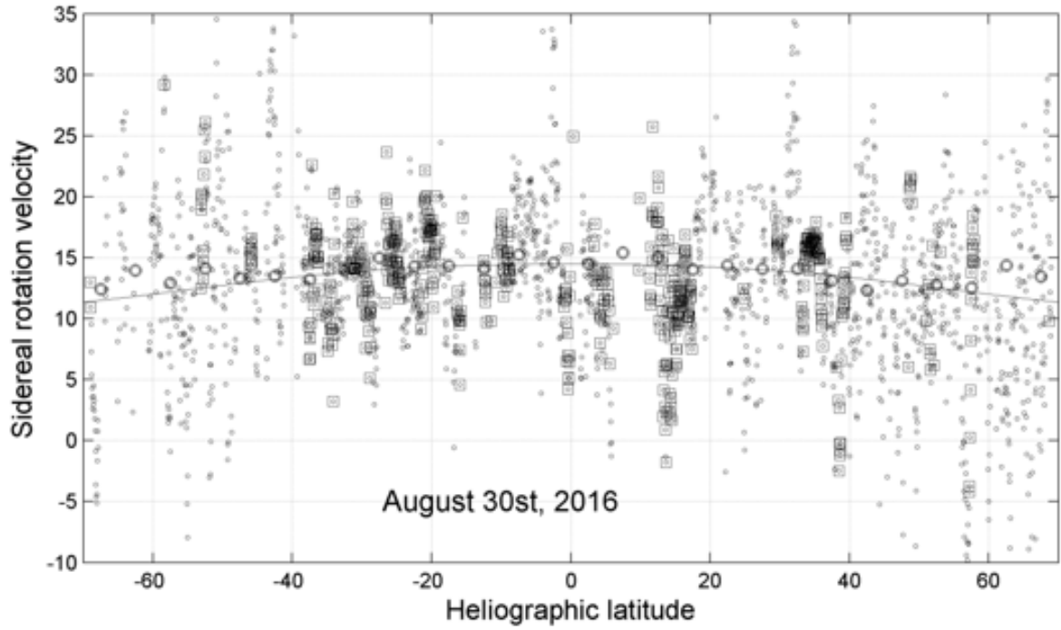
Figure 2.8. Rotational profile as derived using the CC method, where squares mark the mean values in 5° sectors and the solid line is the best fit of these values.
